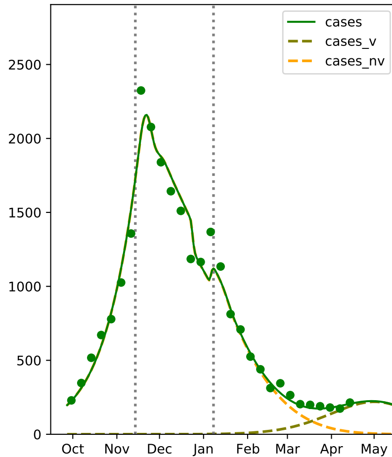
New Mexico: April 18 fit
