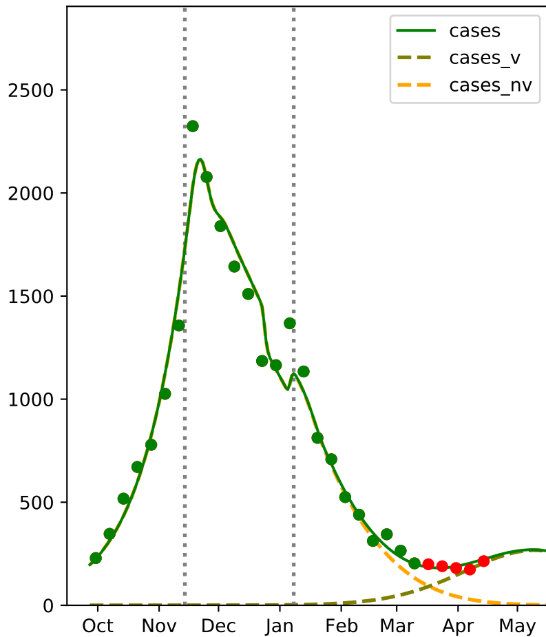
New Mexico: March 16 fit
