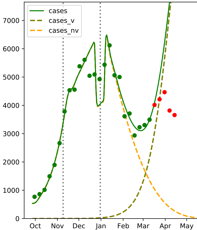
New Jersey: March 16 fit
