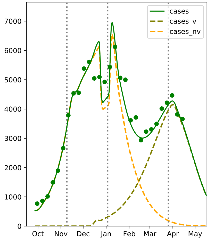
New Jersey: April 18 fit
