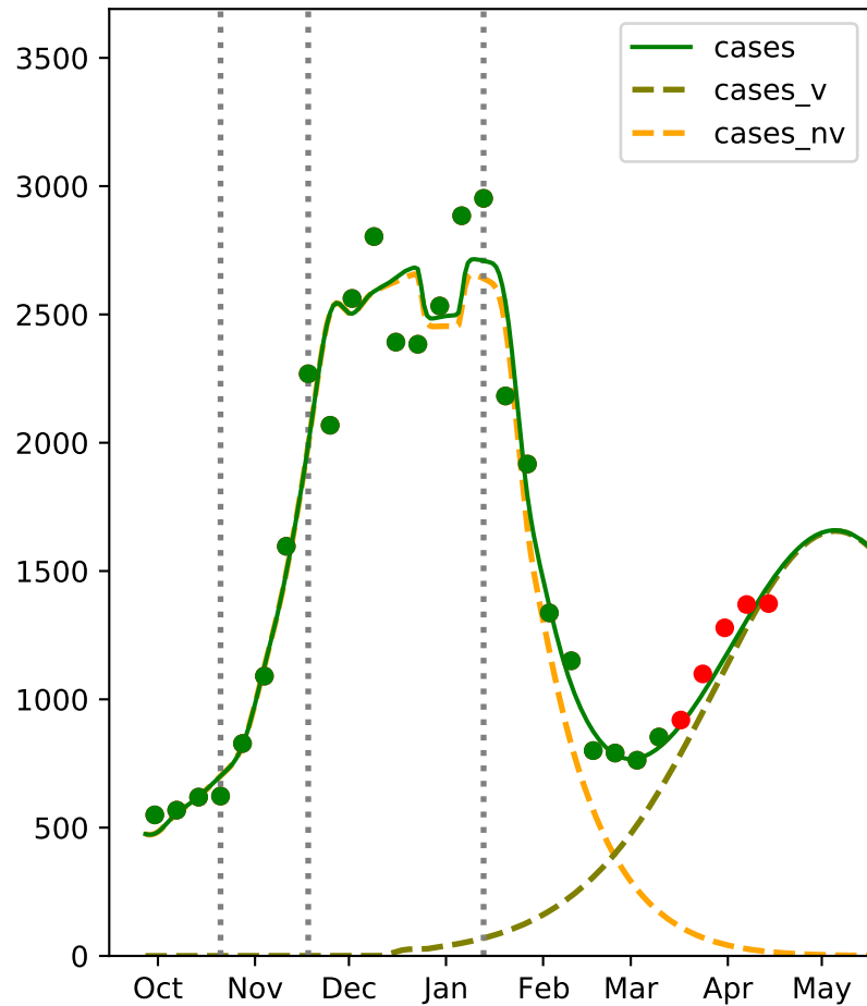
Maryland: March 16 fit
