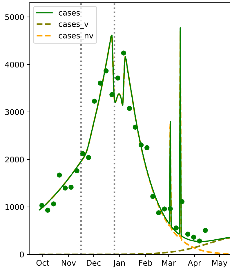
Alabama: April 18 fit
