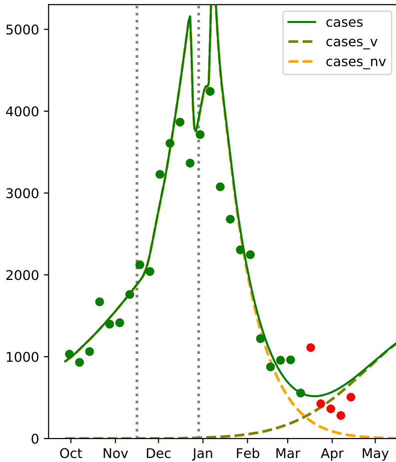
Alabama: March 16 fit
