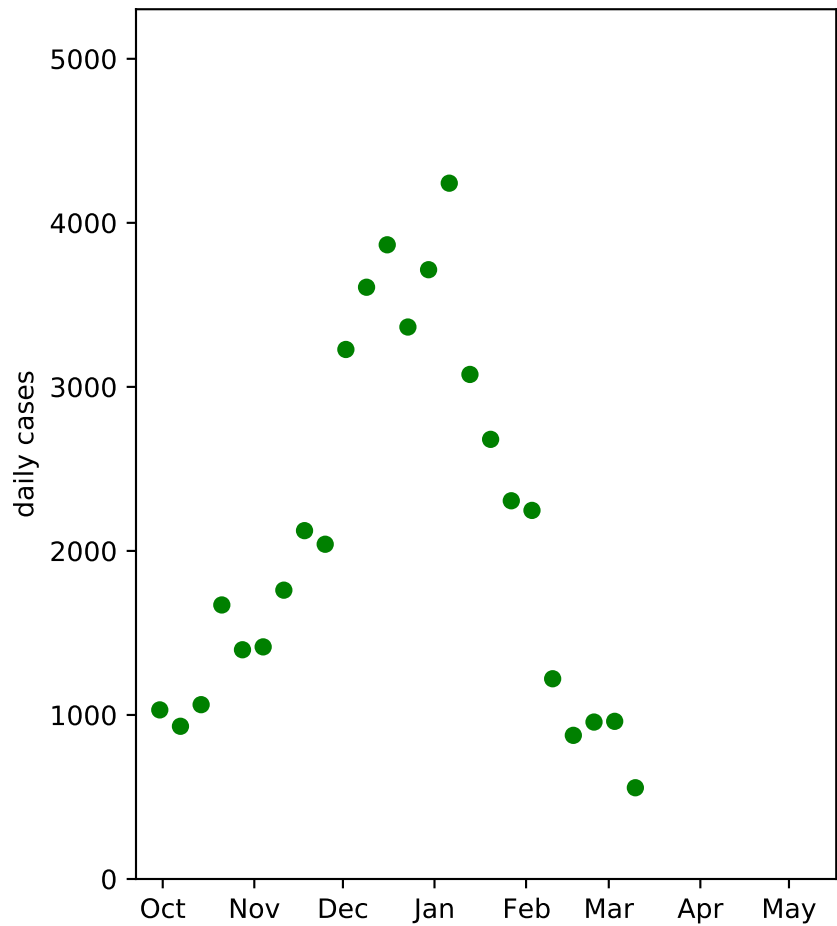
Alabama: March 14 data
